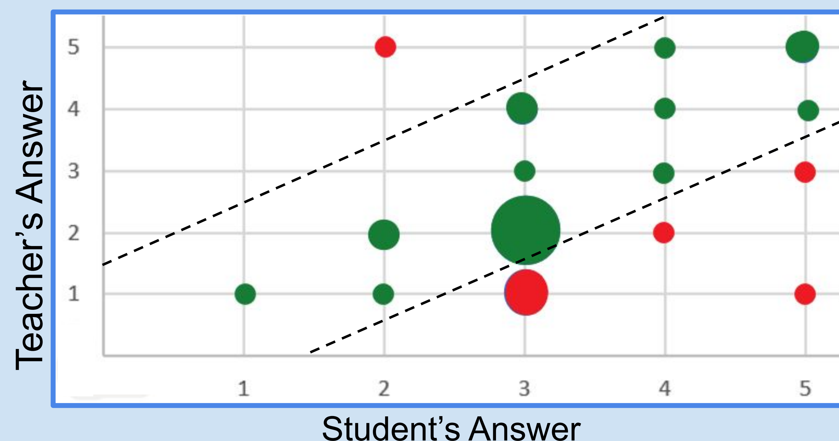
Scatter Plot of Answers
