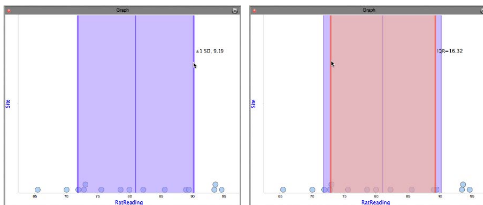
Figure 2: Graphs showing SD (left) and both SD and IQR (right)
