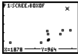
Figure 20: Scatterplot
