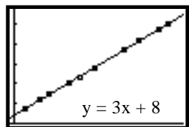
Figure 10: y = 3x + 8
