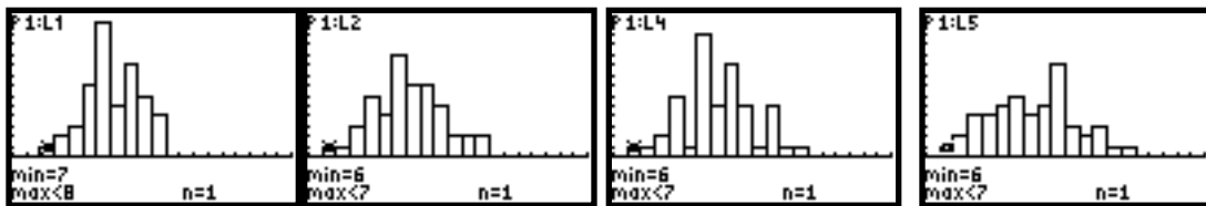
Figure 14: Sampling distributions
