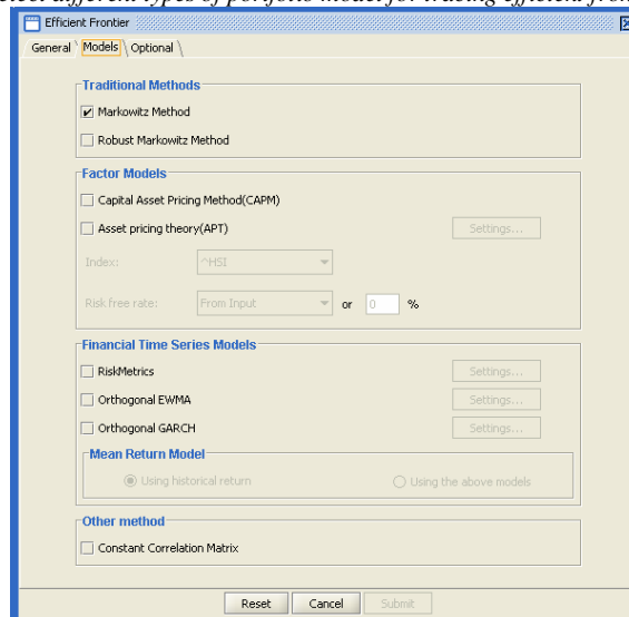
Select different types of portfolio model for tracing efficient frontier
