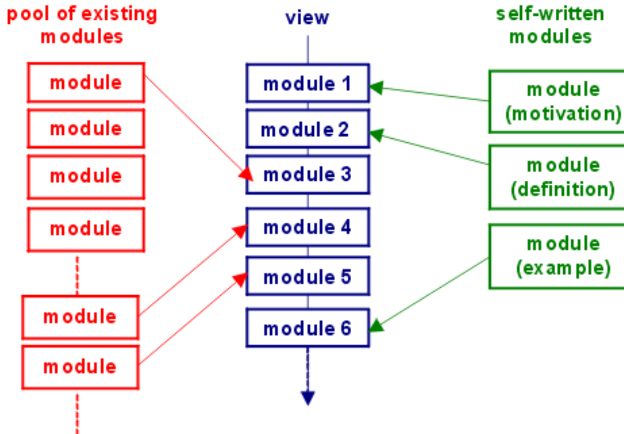
Figure 3: Modules and views in e-stat
