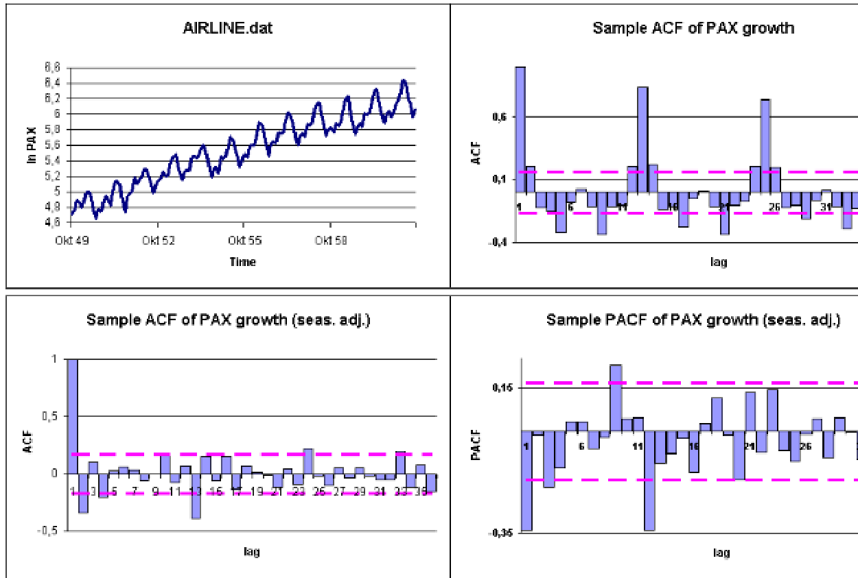
Figure 6: Time Series Analysis with MD*ReX
